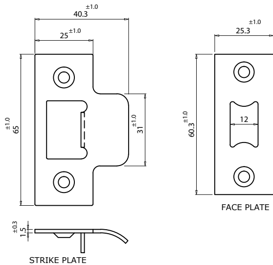
STRIKE PLATE
