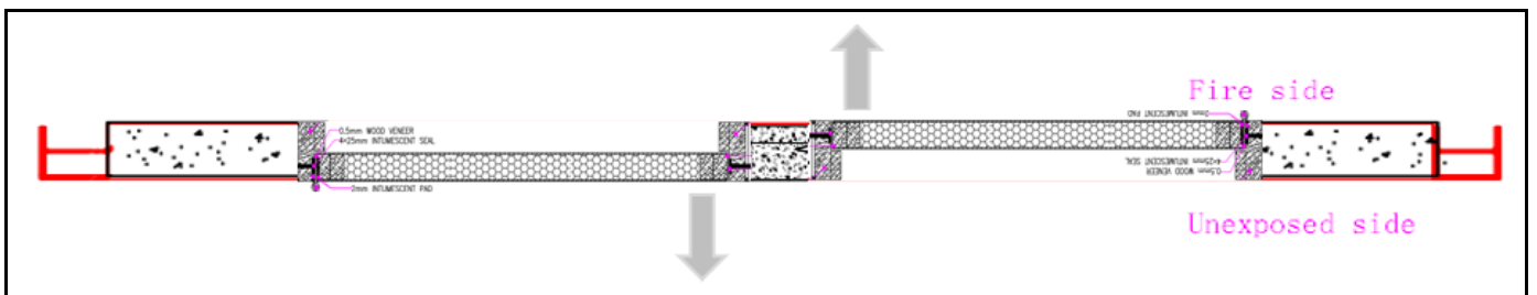
Figure A.2 Supporting Constructions Drawing (Plan view)
