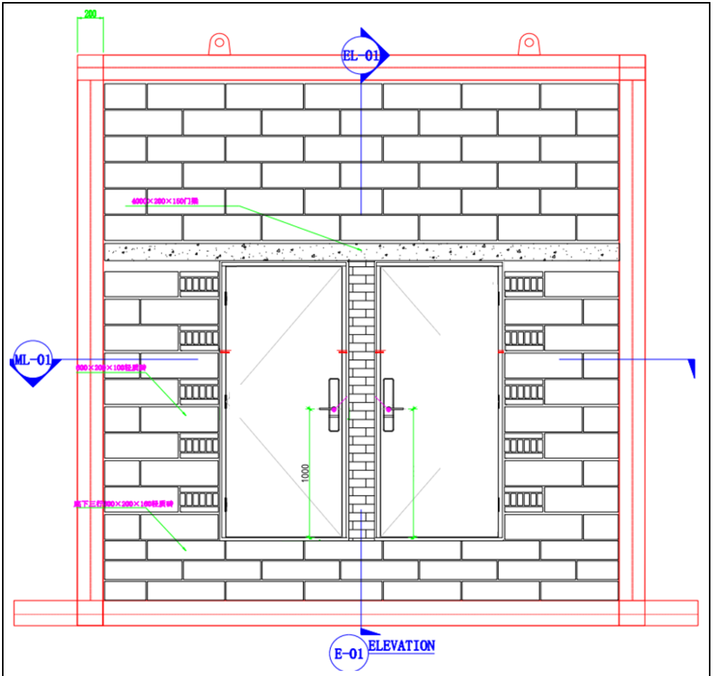
Figure A.1 Supporting Constructions Drawing (View from unexposed side)
