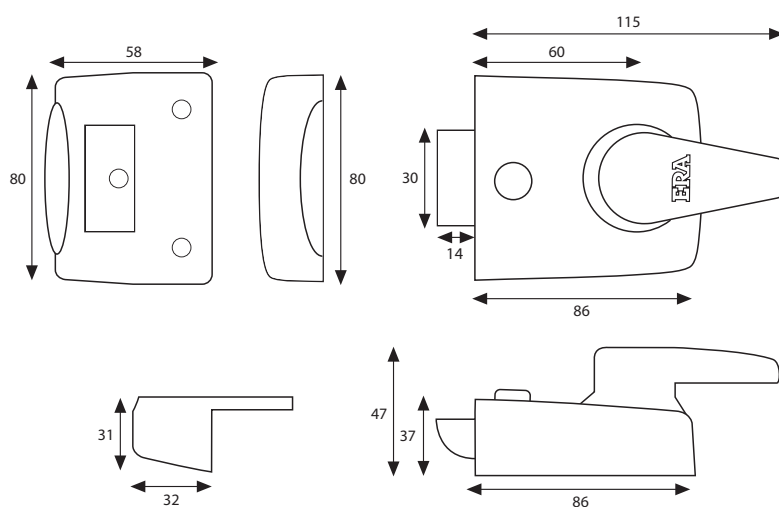
60mm Nightlatch
