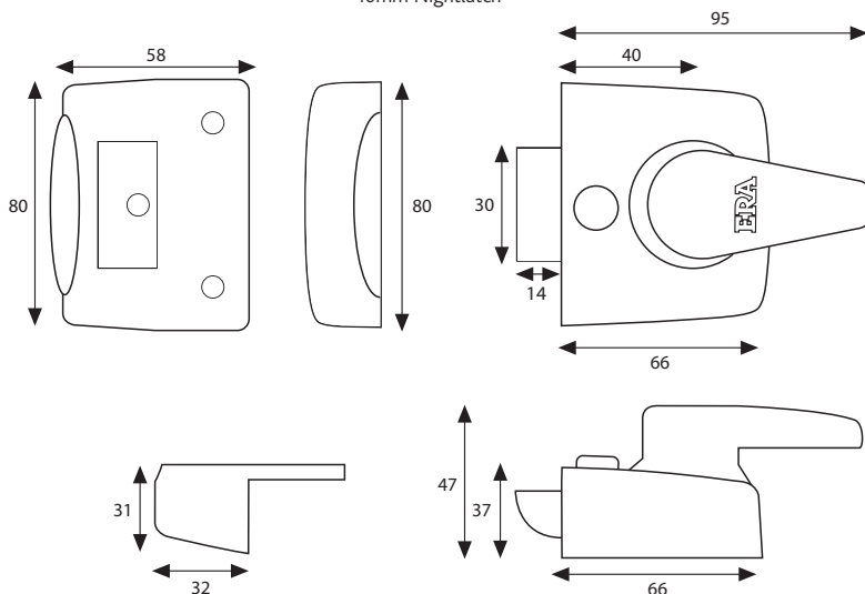
40mm Nightlatch
