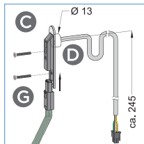
Figure 3.2-2: Detail frame part 2
