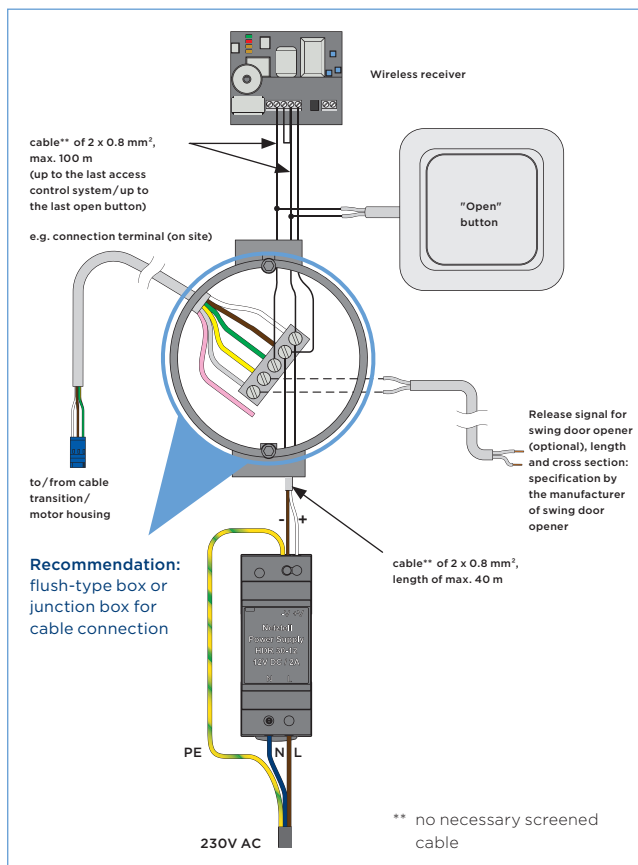
Figure 3.5.1-2: Installing the wireless receiver
