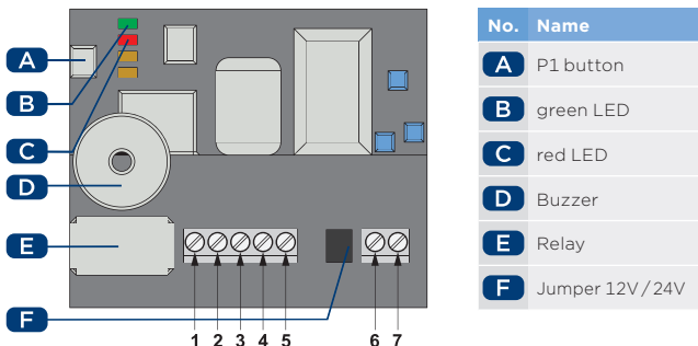
Figure 3.5.1-1: Terminal assignment of the wireless receiver
