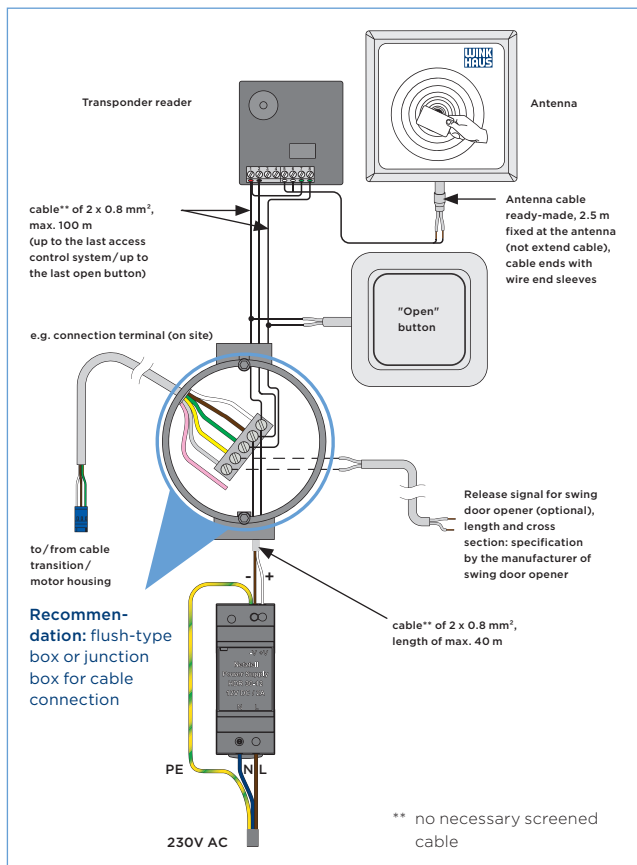
Figure 3.4-2: Installation of the transponder reader
