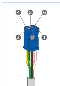
Figure 3.2-4: Cable assignment when used with blueMatic EAV
