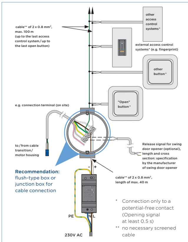
Figure 3.3.1-1: General connection diagram
