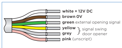
Figure 3.3.1-2: Detail of terminal assignment
