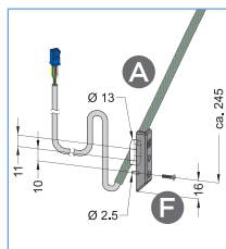
Figure 3.2-3: Detail T-KÜ-T1 FT without cover plate
