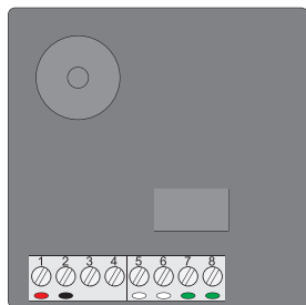
Figure 3.4-1: Terminal assignment of the transponder reader
