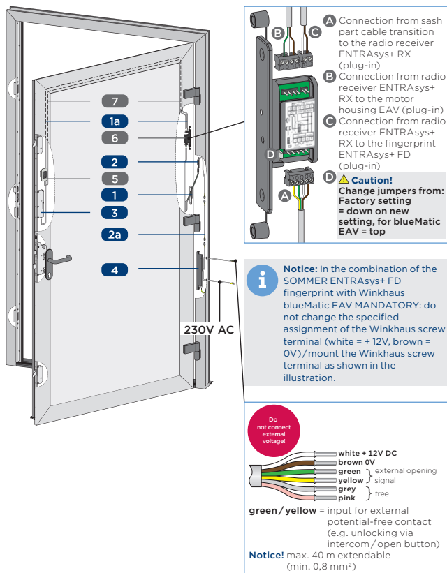
Figure 3.6.2-11: Installation blueMatic EAV with "Fingerpint SOMMER ENTRAsys+ FD and frame power supply" (sash side)
