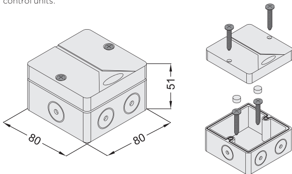
Figure 3.5.2-1: Installing the wireless receiver (dimensions in mm)
