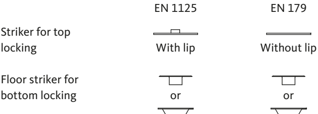
Fig. 2: Approved striker shapes
