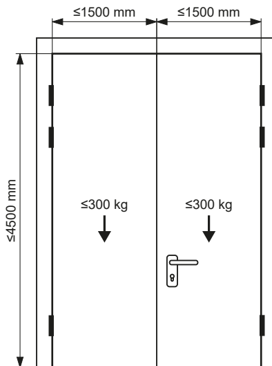
Fig. 3: Max. door dimensions and weights
