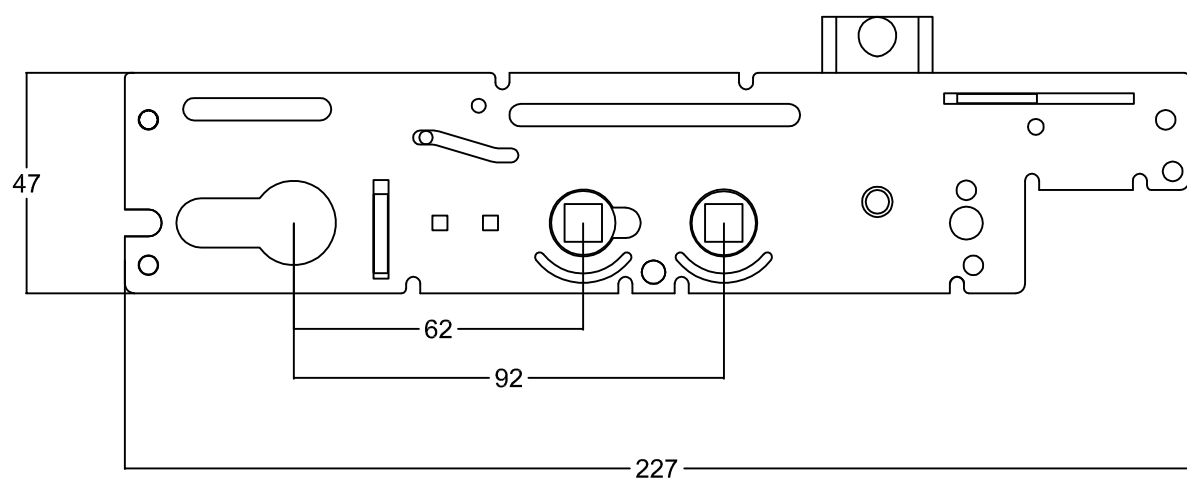
XLCENTRE DUAL SPIN XL 35mm backset centre case dual spindle
