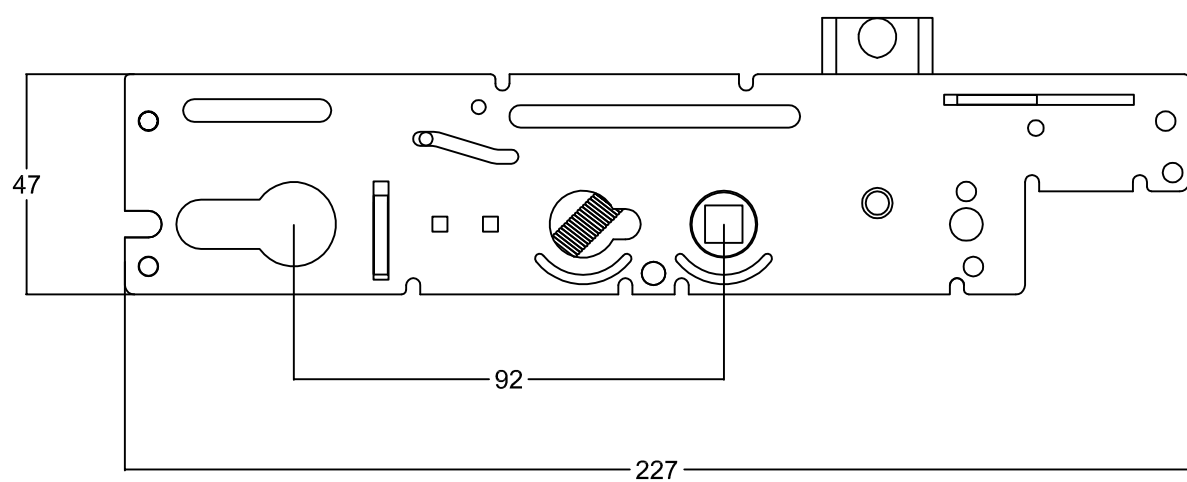
XLCENTRE SINGLE SPIN XL 35mm backset centre case single spindle
