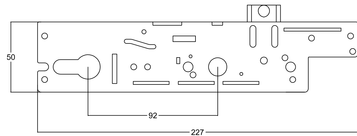
XLCENTRE SPLIT SPIN XL 35mm backset centre case inline split spindle
