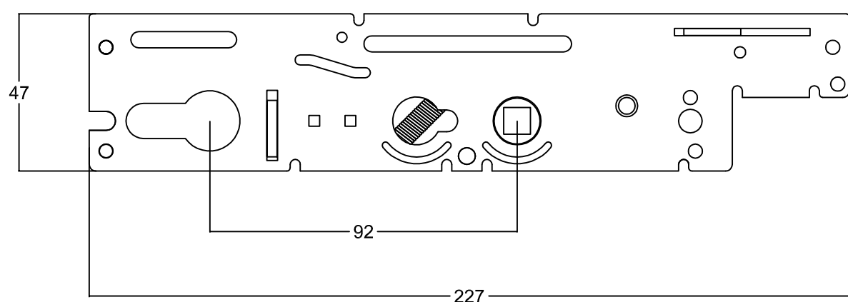
XL CENTRE SLAVE XL 35mm backset centre case slave door
