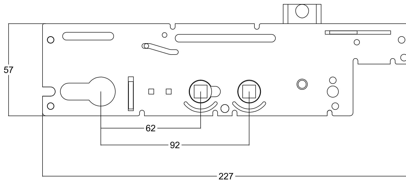
XL CENTRE DUAL 45MM DUAL XL 45mm backset centre case dual spindle
